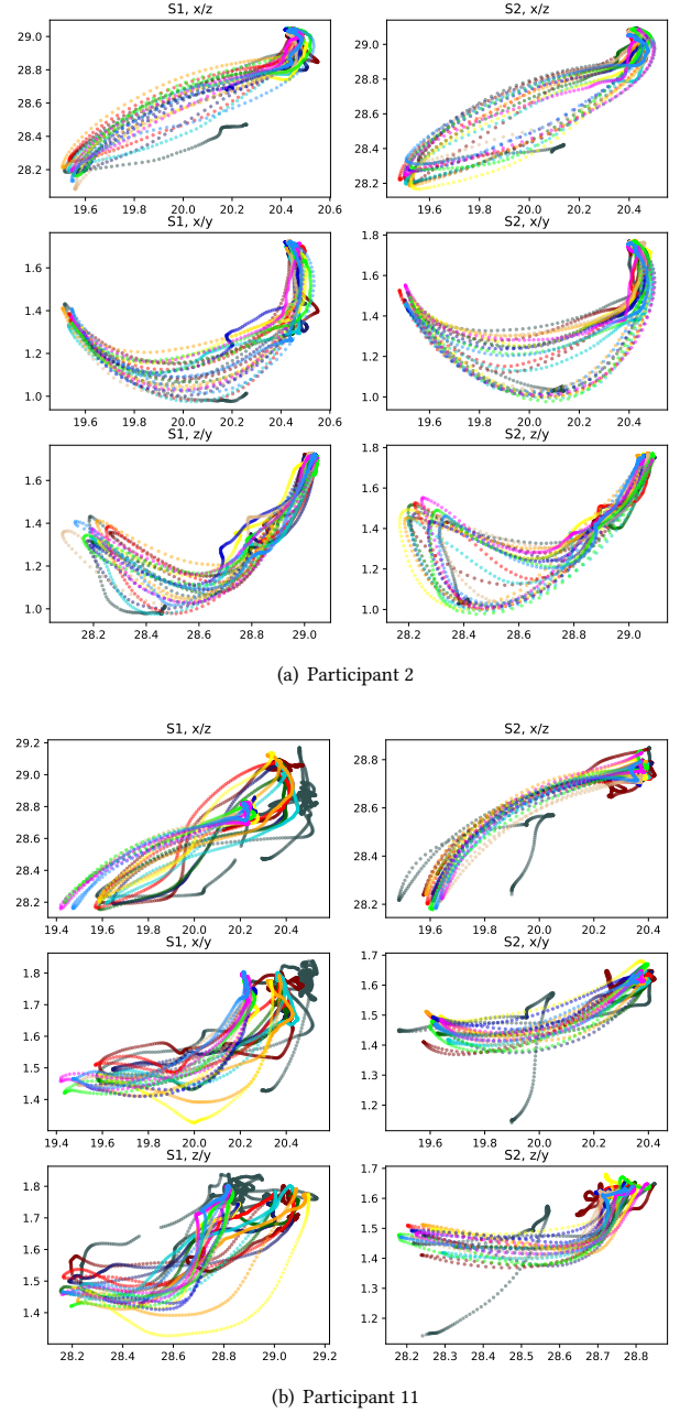
Figure 4: Motion data of the left hand-held controller in the Archery scenario without any applied body normalization for participants 2 and 11 . The axes indicate the global coordinate frame. The colors indicate the repetitions within the study. “S1” and “S2” correspond to the first and second day of the study and “x/z”, “x/y” and “z/y” are the plotted Unity axes (i.e., top view, side view, frontal view). The similarity within each participant is well visible together with the dissimilarity between participants.
